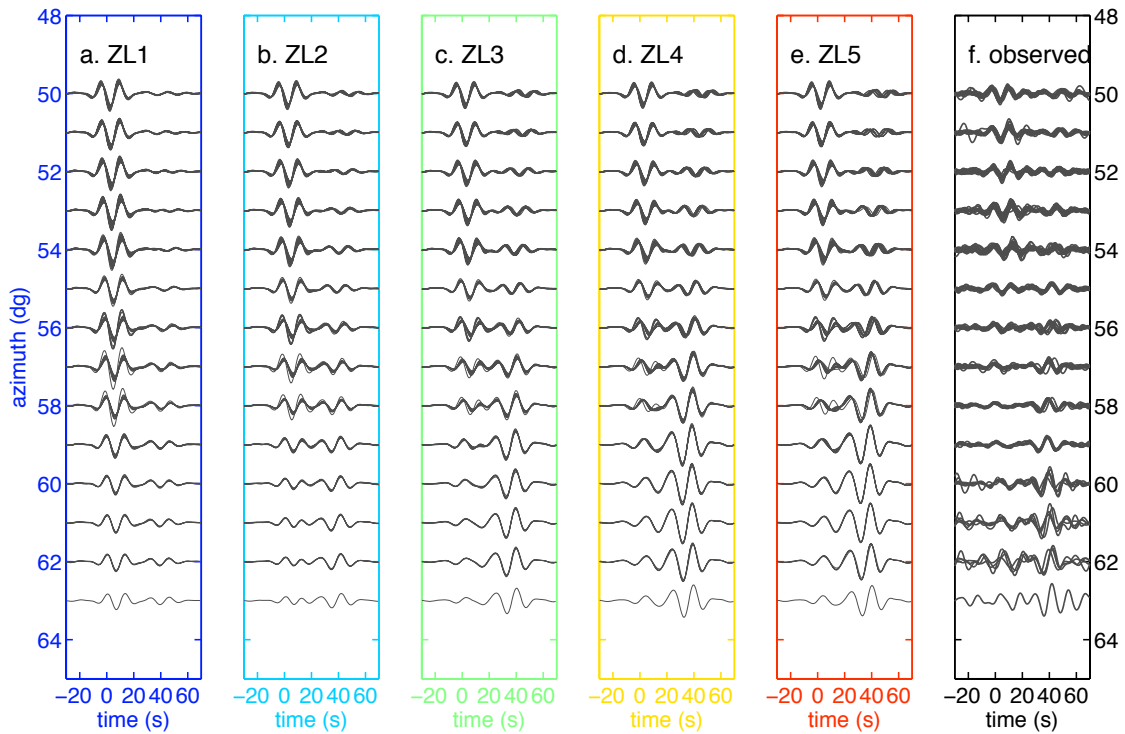
Figure 2.19: Synthetic velocity waveforms are shown in panels a-e correspond to the circular bases in Figure 9 from west to east (as color-coded). Only traces for azimuths above 50^\circ and distances between 100 and 110^\circ are shown. The waveforms are filtered between 10 and 20 s. The last panel (f) shows the observed data for comparison. From left to right, or geographically from west to east, more of the ULVZ lies within the diffracted path and amplitude or the postcursor increases. Additionally there is some variation in amplitude of the main phase between the different models. Our final model sits between ZL2 and ZL3.
