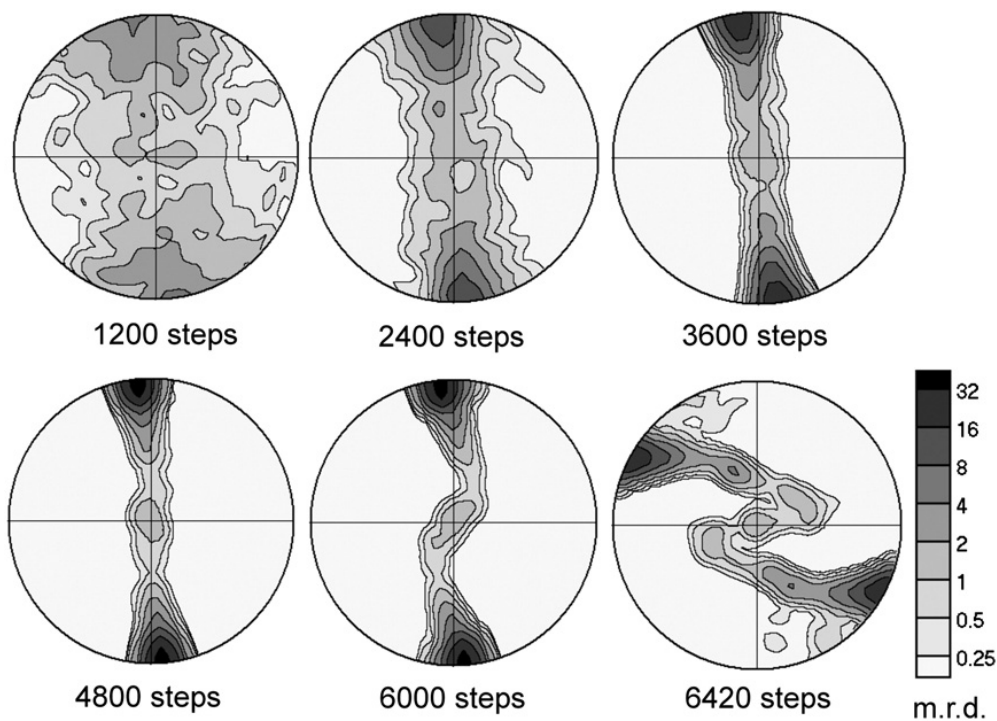
Figure 5.7: Resulting textures or preferred orientation showing the density of (001) poles as a equal area contour plot (scale is quadratic). This texture development is along the lowermost tracer for pPv C (001). A rotation of the final texture occurs at the final time step plotted (where the tracer enters an upwelling). Figure courtesy of Rudy Wenk.
