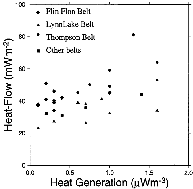
Figure 3. Heat flow and heat production data. The data from the Flin Flon-Snow Lake, Thompson and Lynn Lake belts are identified.
