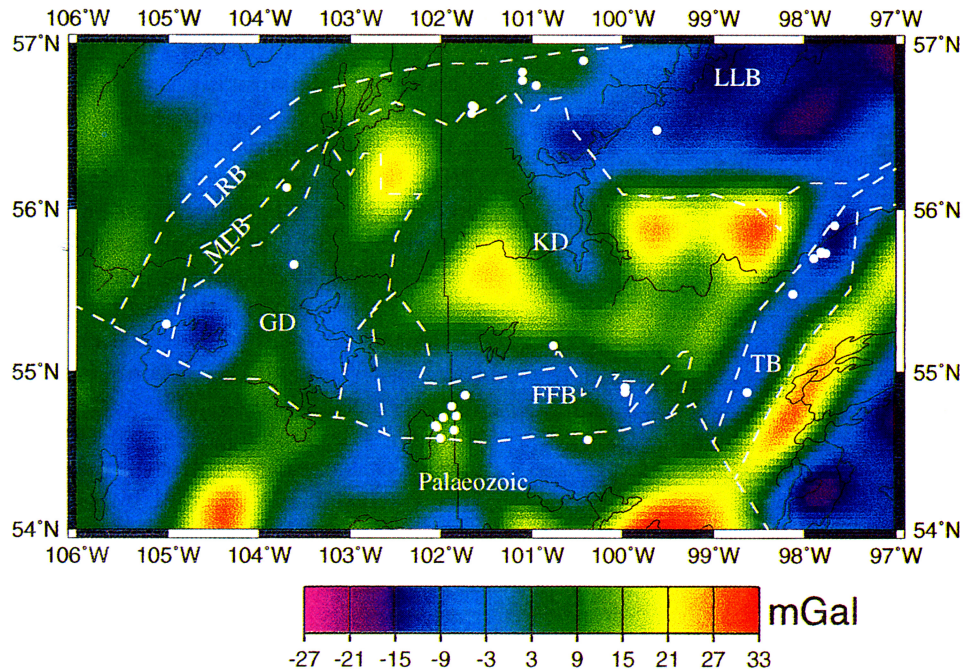
Plate 2. Filtered gravity map of the study area. Wavelengths shorter than 50 km have been eliminated and wavelengths longer than 80 km have not been modified. The main tectonic belts in the Reindeer zone are superposed: GD: Glennie domain, FFB: Flin Flon-Snow Lake belt, KD: Kisseynew domain, LLB: Lynn Lake belt, LRB: La Ronge Belt, TB: Thompson belt. Gravity data are from the Geomatics Canada database. The white circles indicate the location of the heat flow sites.
