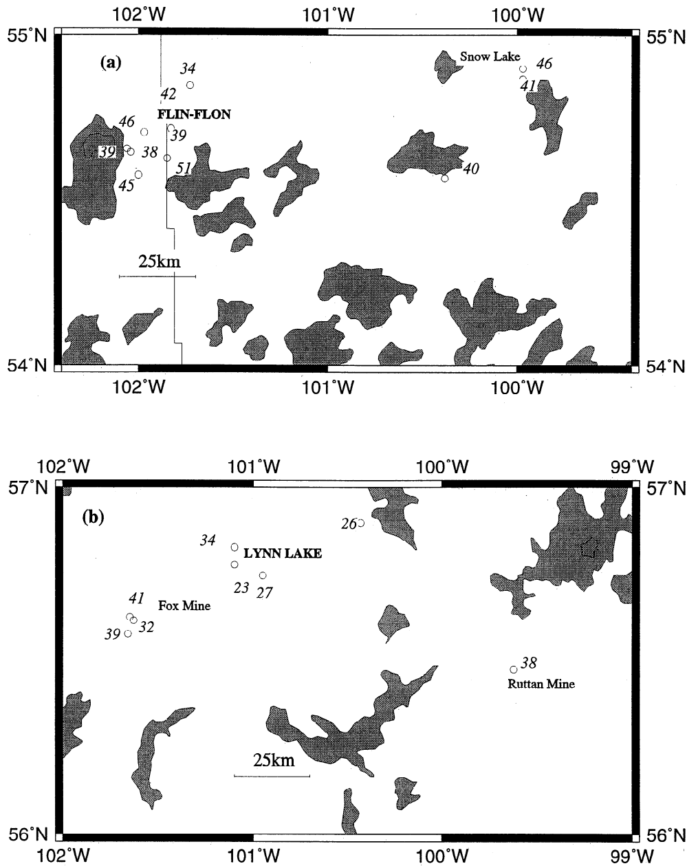
Figure 4. Local variations in heat flow values: (a) in the Flin Flon-Snow Lake belt, and (b) in the Lynn Lake belt. Heat flow values are in \text{mW m}^{-2} .
