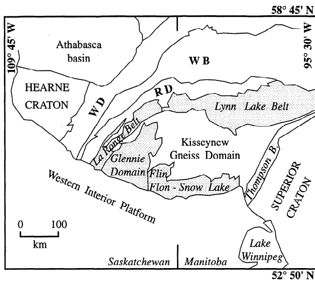
Figure 1. Geological map of the exposed Trans-Hudson Orogen in Manitoba and Saskatchewan, adapted from [Lucas et al. , 1996]. RD is the Rotenstone domain, WB is the Wathaman batholith, and WD is the Wollaston fold belt. Juvenile Proterozoic crust is exposed in the Reindeer tectonic zone including the Rotenstone, La Ronge-Lynn Lake, Glennie, Kisseynew, and Flin Flon-Snow Lake domains.
