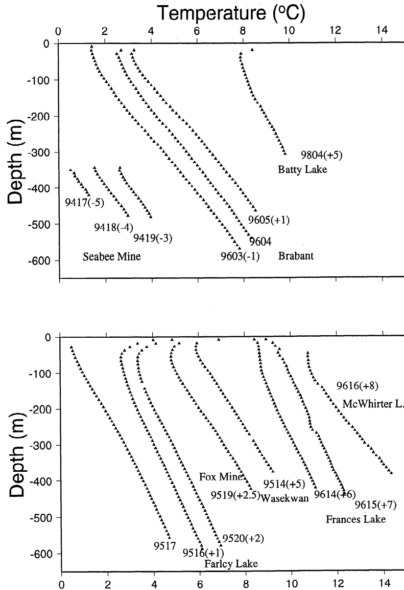
Figure 2. Measured temperature profiles for all the sites. For clarity, temperature profiles are shifted as indicated.
