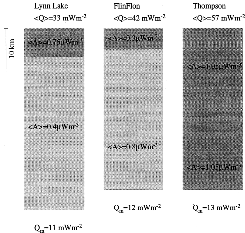
Figure 5. Average crustal column for the Lynn Lake, Flin Flon, and Thompson belts. Crustal thickness for Flin Flon and Lynn Lake is constrained by seismic data. Beneath the surficial layer, the crust is depleted for Lynn Lake, average for Flin Flon-Snow Lake, and enriched for Thompson.
